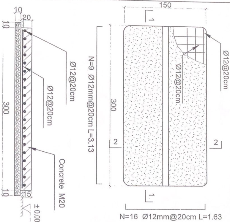
1-1 section
