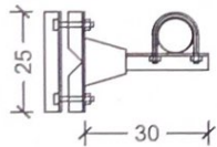
TYP 1M ANTENNA SUPPORT
